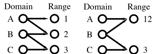
Figure 3: shows a global substitution: range elements 1 and 2 are merged, preserving all links. It is called a global substitution as every link with 1 or 2 in the range now has 12 as its range element.
